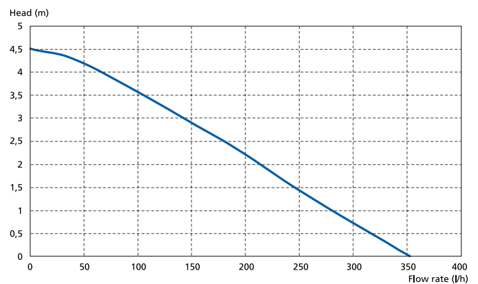
Kondensat-Lift characteristic curve
